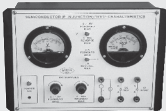
P-N JUNCTION DIODE TRAINER
